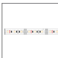
LED pásek K-1275- RGB-12V 14.4W/m Ref: K-1275-RGB-12V
