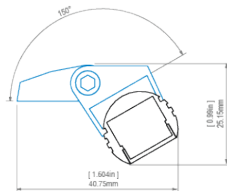
PDS-O profile and REG-PD-UV mounting bracket profil PDS-O z mocovníkem REG-PD-UV
