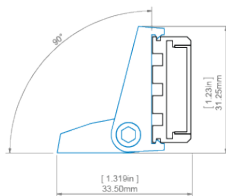
GIZA profile and REGIP-UV mounting bracket profil GIZA z mocowníkem REGIP-UV
