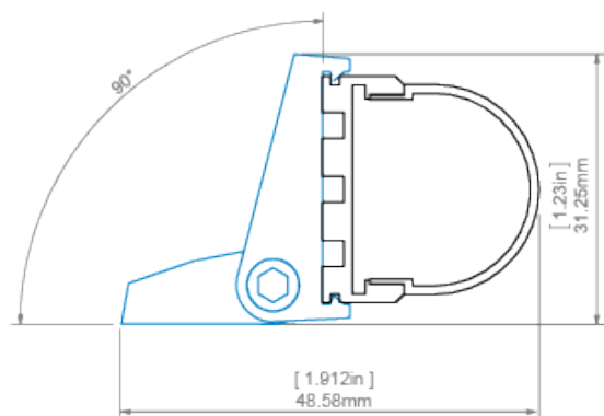
GIZA profile with G-L cover and REGIP-UV mounting bracket profil GIZA z oslönou G-L oraz mocovníkem REGIP-UV
