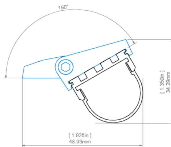
GIZA profile with G-L cover and REGIP-UV mounting bracket profil GIZA z oslönou G-L oraz mocovníkem REGIP-UV
